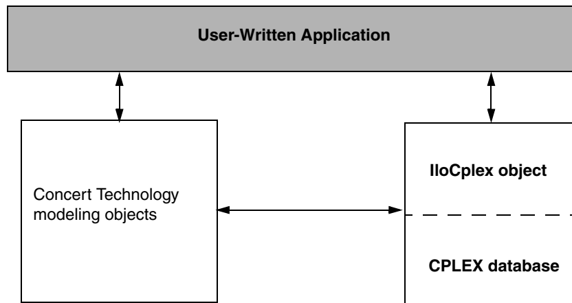
Figure 2.1 A View of ILOG CPLEX with ILOG Concert Technology
