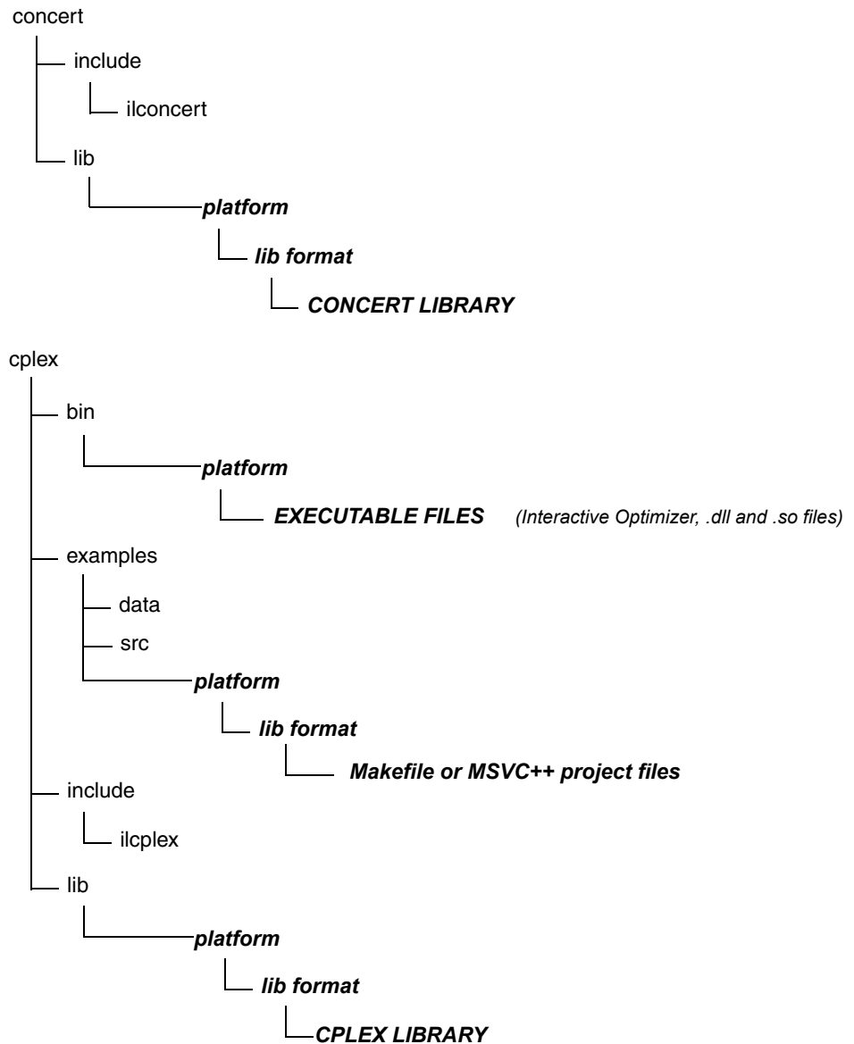
Figure 1.1 Structure of the installation directory
