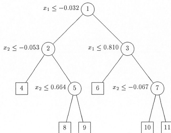
Figure 4: Pruned tree for logistic regression example.
