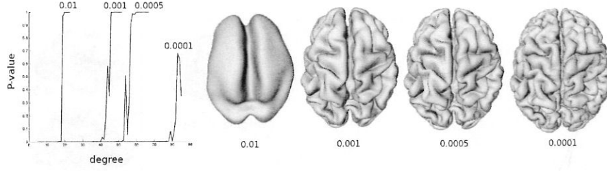
Figure 2: Automatic degree selection in the IRF algorithm. For each band-width t , the optimal degree is automatically selected by checking if adding an additional degree will be statistically significant. The outer cortical surfaces are the results of the optimal selection procedure. The optimal degrees are k = 18(t = 0.01) , k = 42(t = 0.001) , k = 52(t = 0.0005) , k = 78(t = 0.0001) . For our study, t = 0.0001 and the corresponding degree k = 78 is used through the paper.
