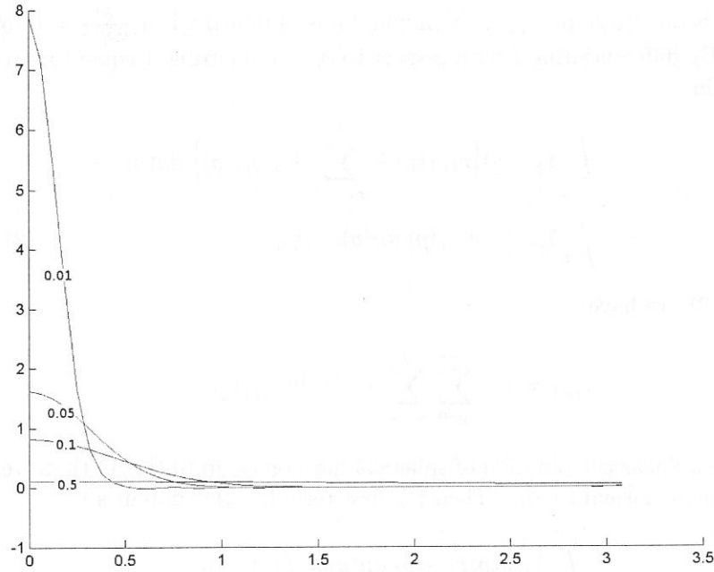
Figure 3: Shape of heat kernel with different bandwidth t = 0.01, 0.05, 0.1, 0.5 . The horizontal axis is the \theta value from the north pole ( \theta = 0 ) to the south pole ( \theta = \pi ). The weighting scheme used in WFS follows the shape of the heat kernel.
