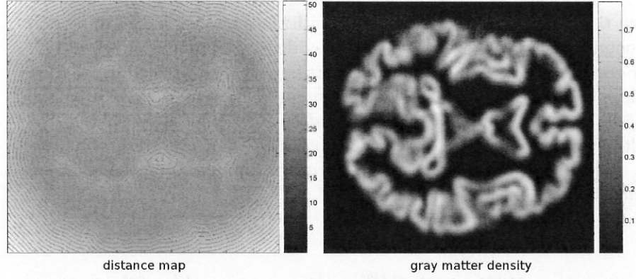
Figure 8: Left: contour plot of the average distance map in mm at scale \alpha = 0 . Right: Gaussian kernel smoothing of the gray matter density map with 10mm FWHM.
