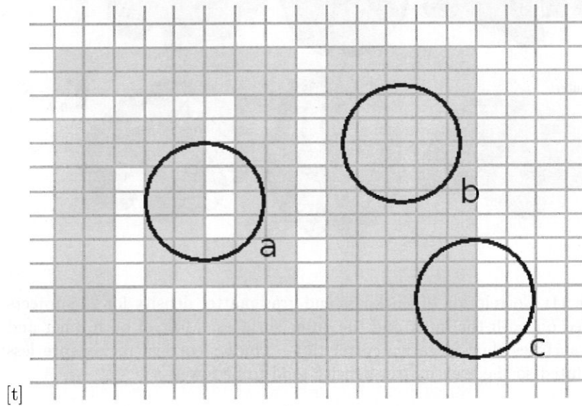
Figure 12: Simple 2D schematic showing the negative correlation between thickness and gray matter density. Gray colored pixels are the gray matter. The black circles are the contour of heat kernel. There are less gray matter pixels in region (c) than region (a) although the thickness in region (c) is thicker than that of region (a). The gray matter density in the middle of the gray matter (b) is close to 1 for all subject indicating very small between-subject and between-group variability. Because of the small between-group variability, VBM does not usually detect signal in the middle of the gray matter. Most of the significant signal detected in VBM is near the tissue boundary where the between-group variability is high.
