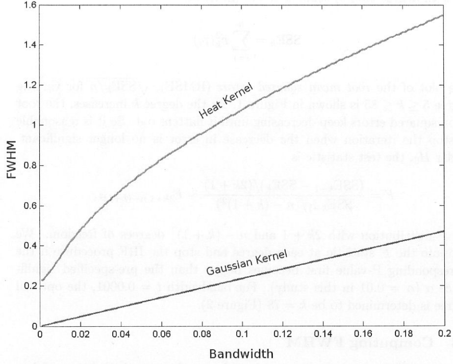
Figure 4: Plot of FWHM (vertical) over bandwidth t (horizontal) for both heat kernel and Gaussian kernel. The FWHM has to be numerically estimated in the case of the heat kernel. The numerically computed FWHM is used in the random field theory based multiple comparison correction.
